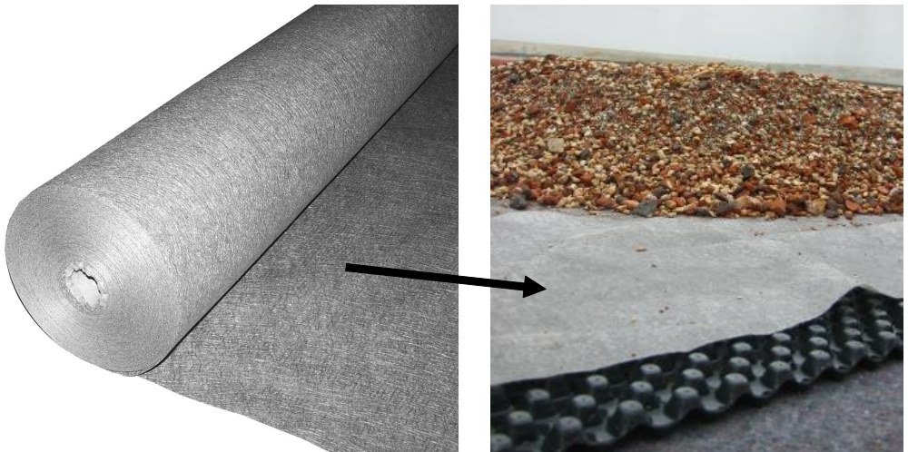
Figure 1 & 2 Filter sheet and its typical location within the build-up of the green roof system.
